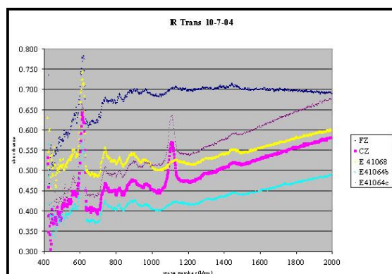
Figure 1. FTIR spectra of CZ and FZ control samples as well as three unknown pieces recovered from the Genesis payload.
